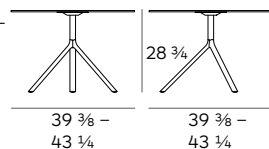
Mod. 9555-01 (Ø 39 3/8) Mod. 9556-01 (Ø 43 1/4)
