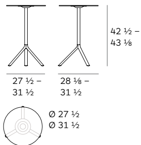
Mod. 9590-71 (Ø 27 1/2) Mod. 9591-71 (Ø 31 1/2)
